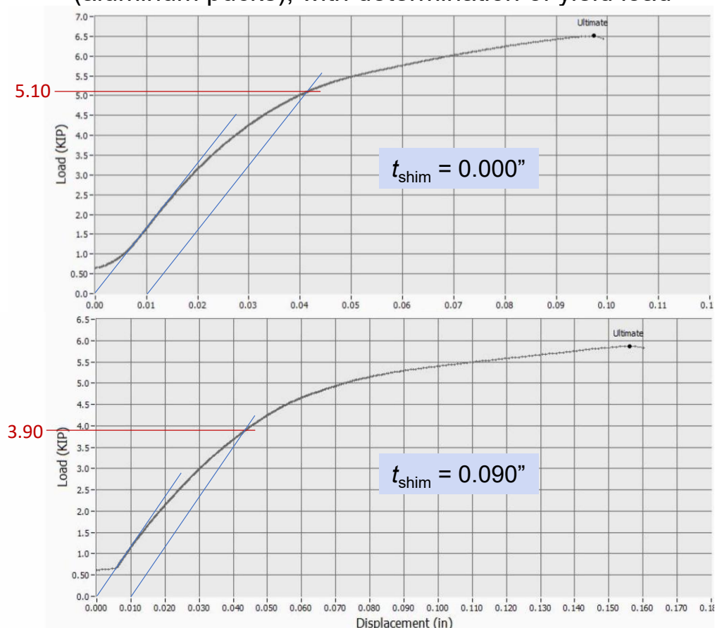
Representative load-displacement plots from Ref. 13 (aluminum pucks), with determination of yield load
