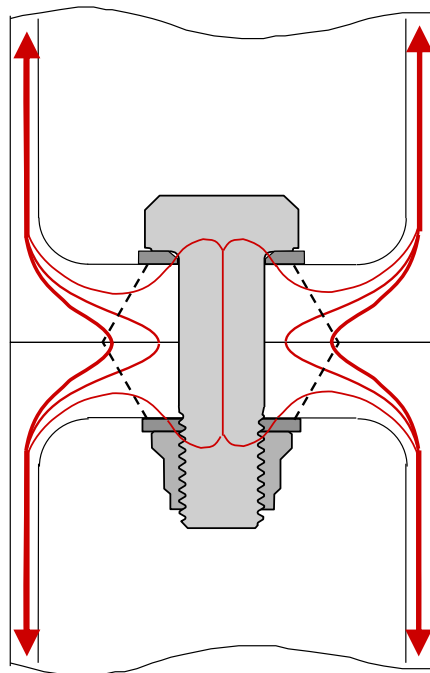
Applied tension
