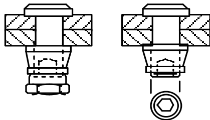
Threaded pin-riquet (Hi-Lok®)
