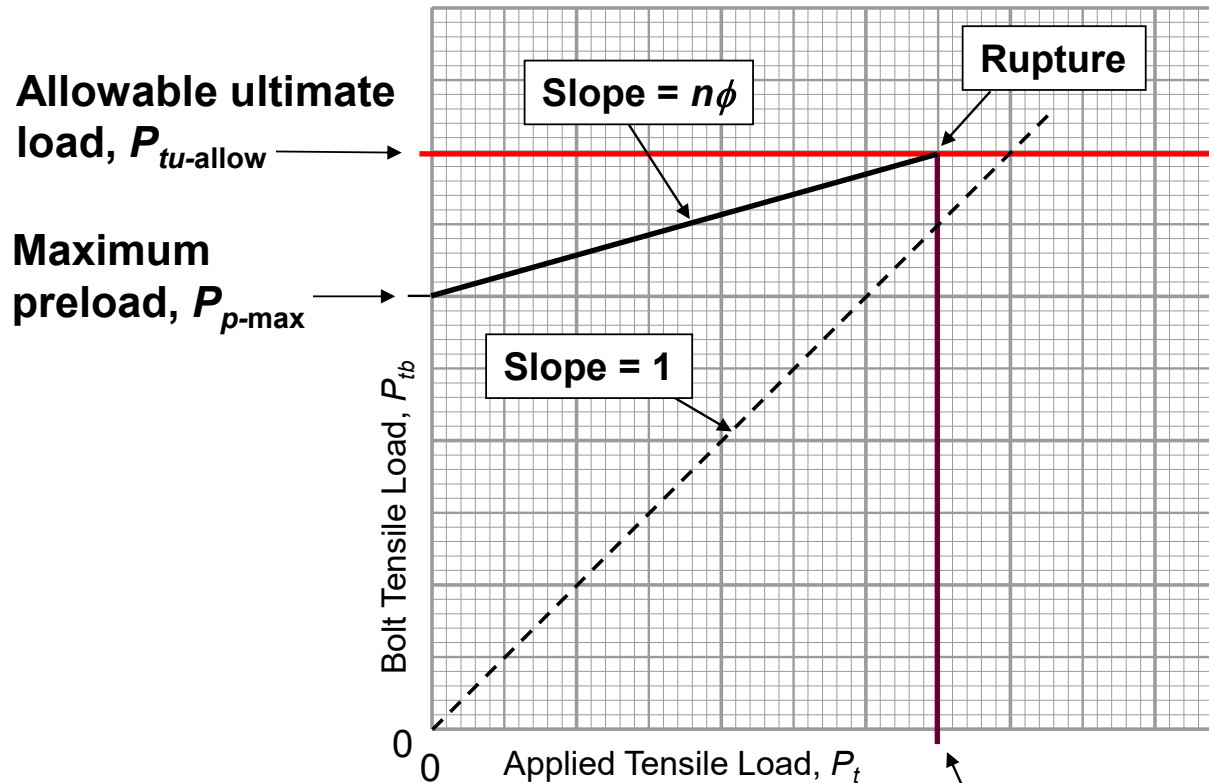
Fig. 9-3 (similar to NASA-STD-5020B Fig. 15)
