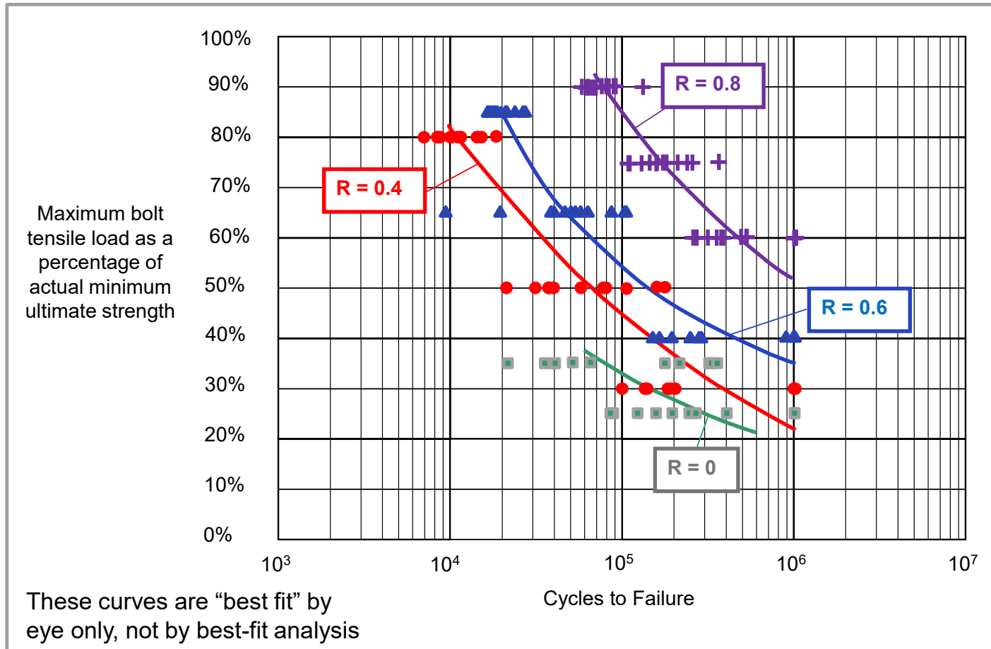
Fig. 9-18. Fatigue Data for NAS 1351N (A-286) Fasteners
