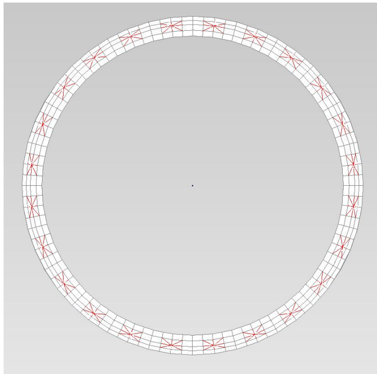
RBE2 spiders at bolt locations shown in red
